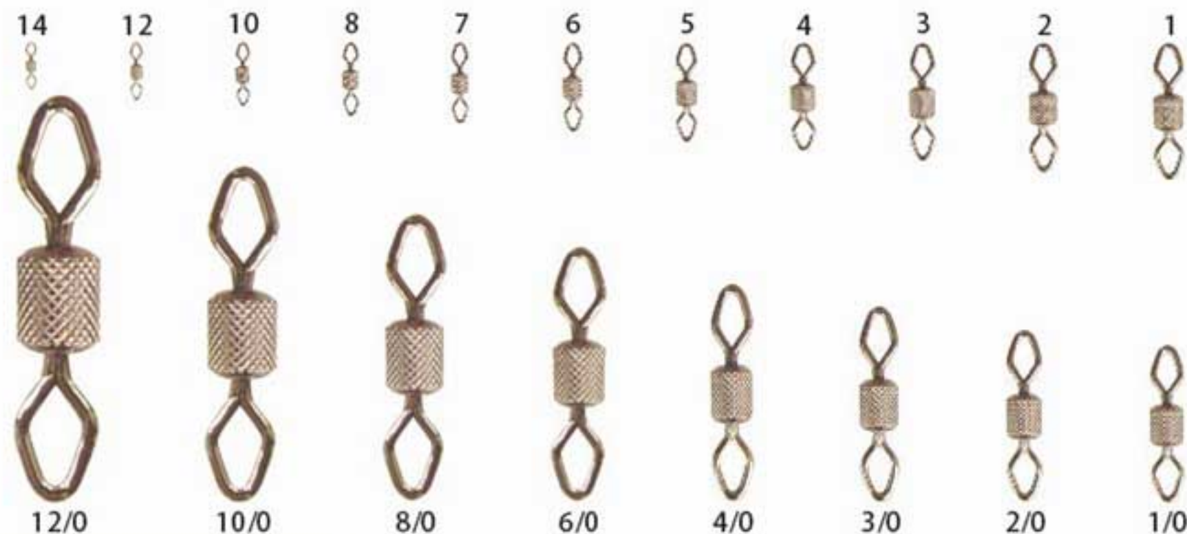
美式菱形压花转环 ZPY-1041 Diamond eye impressed rolling swivel
